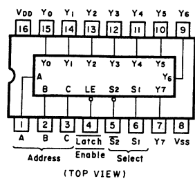
Fig. 7.1.6 3-to-8 Line Decoder IC μPD74HC237
